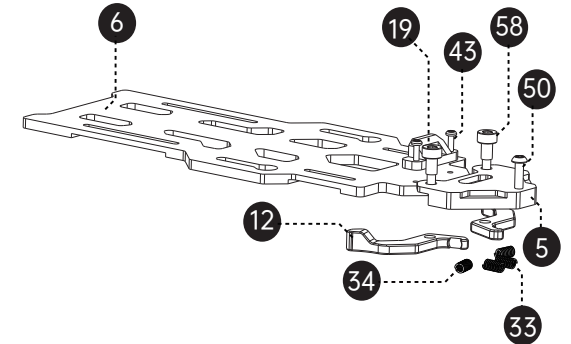
电池固定板 Battery QR Mount
