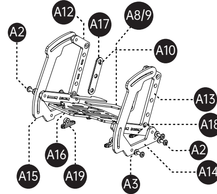
ZCAM 相机套件 ZCAM camera Kit
